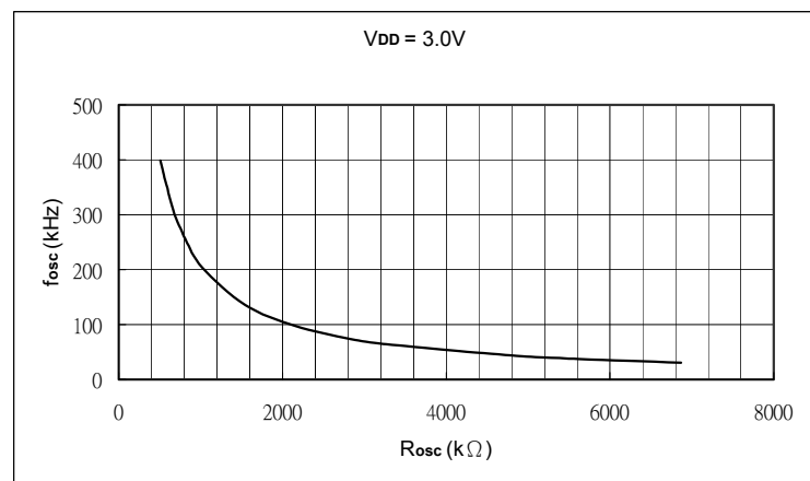
Resistor vs. f_{osc} , V_{DD} = 3.0V
