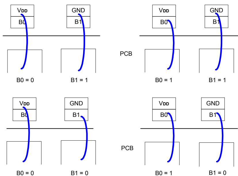
SH66L10A Bonding Option
